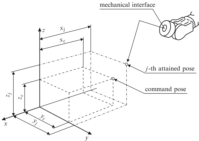
Fig. 9.10 The command and the attained end-effector pose
