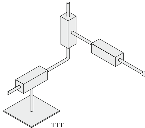
Fig. 1.10 Cartesian robot arm
