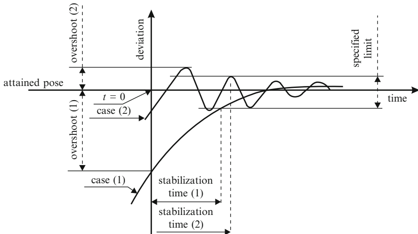
Fig. 9.14 Pose stabilization time and overshoot
