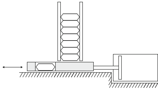
Fig. 8.13 Magazine feeder
