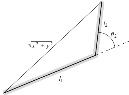
Fig. 4.2 Calculation of the \vartheta_2 angle
