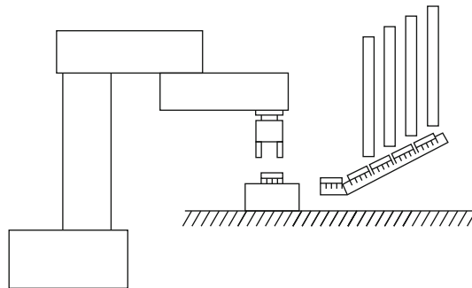
Fig. 8.14 Integrated circuit magazine feeder
